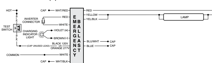
FIG N ONE (1) 21 W - 55 W LAMP WITHOUT AC BALLAST
