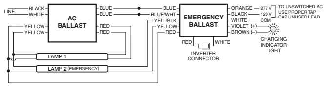
FIG D TWO (2) LAMP RAPID START BALLAST
