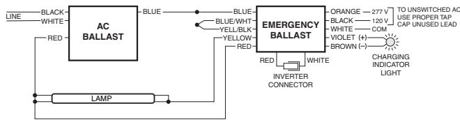
FIG A ONE (1) LAMP INSTANT START BALLAST
