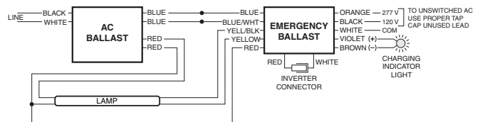
FIG B ONE (1) LAMP RAPID START BALLAST
