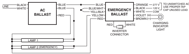
FIG C TWO (2) LAMP INSTANT START BALLAST
