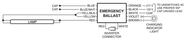
FIG I ONE (1) 17-215 W LAMP WITHOUT AC BALLAST
