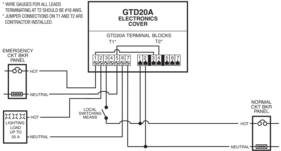
GTD20A as a Generator Transfer Device
