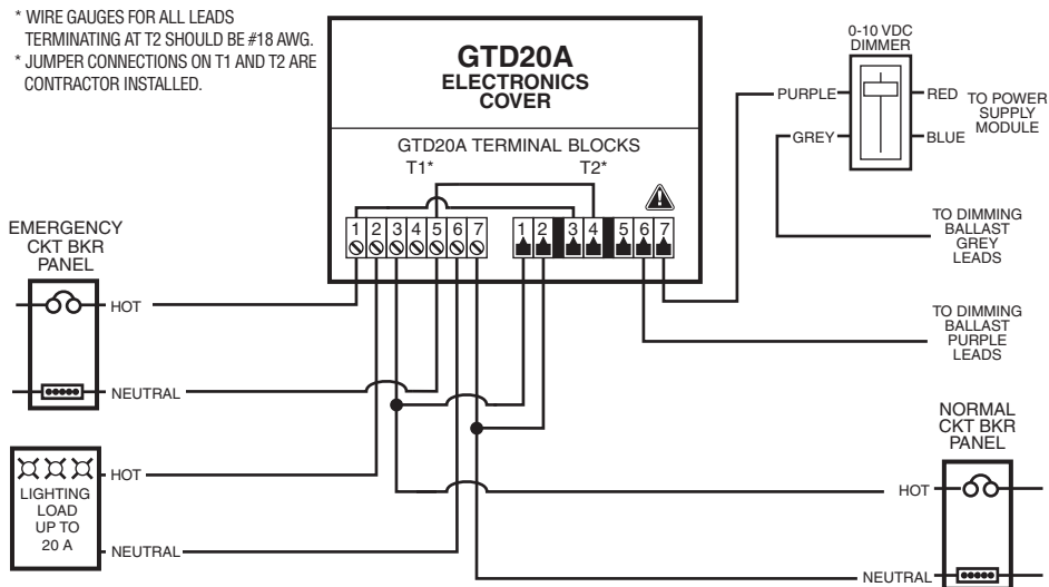
GTD20A as a Generator Transfer Device with a 0-10 VDC Dimming System
