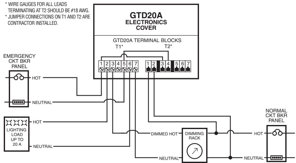
GTD20A as a Generator Transfer Device for a Dimming Rack
