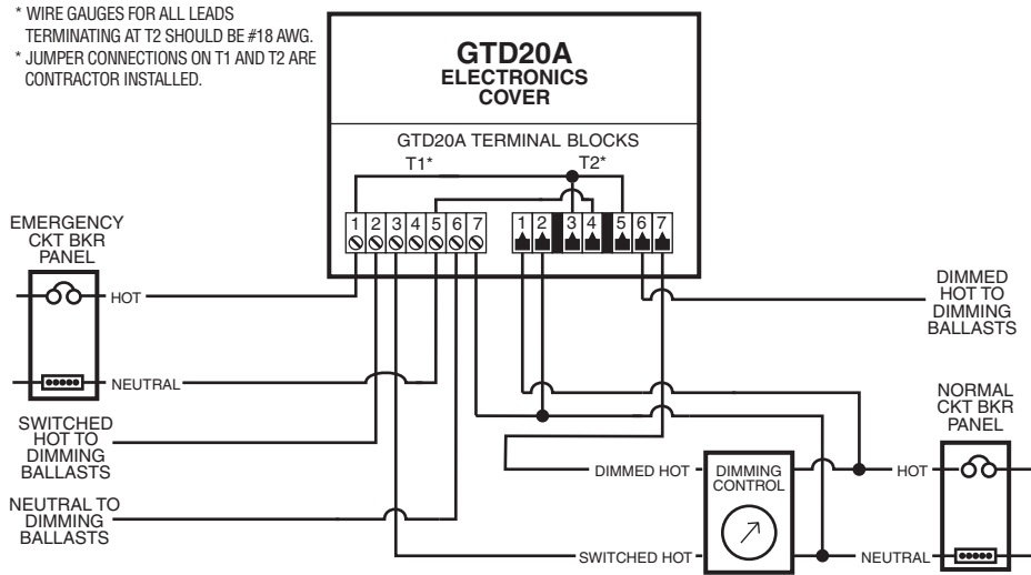
GTD20A as a Generator Transfer Device with a 3-wire Dimming System
