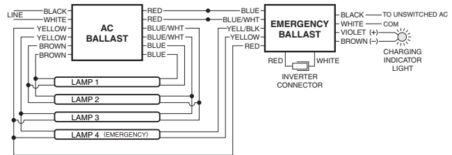
FIG 51a SV FOUR (4) LAMP RAPID START BALLAST
