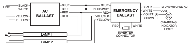
FIG 3b SV TWO (2) LAMP RAPID START BALLAST
