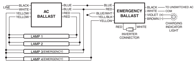
FIG 14b SV FOUR (4) LAMP INSTANT START BALLAST
