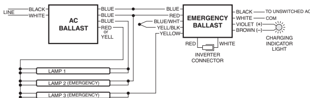
FIG 7b SV THREE (3) LAMP INSTANT START BALLAST
