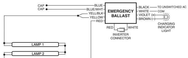
FIG 1b SV TWO (2) 17-40 W LAMPS WITHOUT AC BALLAST
