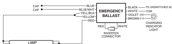
FIG 1a SV ONE (1) 17-215 W LAMP WITHOUT AC BALLAST
