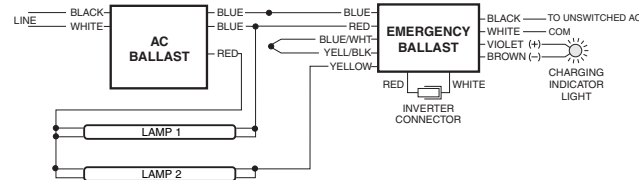
FIG 36b SV TWO (2) LAMP INSTANT START BALLAST
