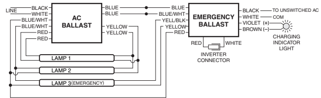
FIG 15a SV THREE (3) LAMP RAPID START BALLAST
