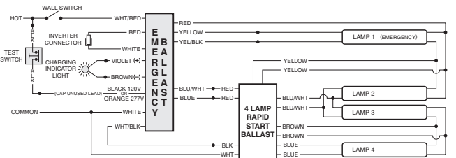
FIG I FOUR (4) LAMP RAPID START BALLAST
