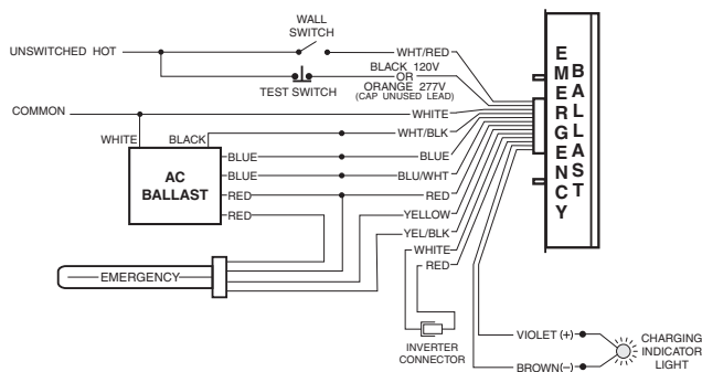
ONE (1) 4-PIN COMPACT LAMP RAPID START BALLAST
