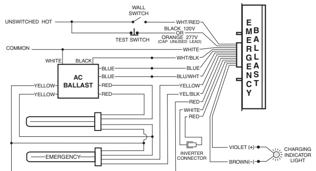
TWO (2) 4-PIN COMPACT LAMP RAPID START BALLAST
