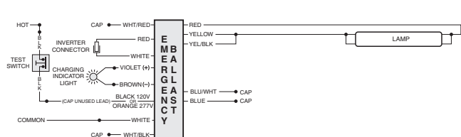
FIG J ONE (1) 17-40 W LAMP WITHOUT AC BALLAST
