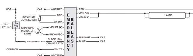
FIG J ONE (1) 17-215 W LAMP WITHOUT AC BALLAST
