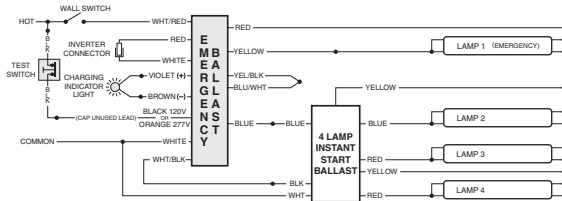
FIG E FOUR (4) LAMP INSTANT START BALLAST
