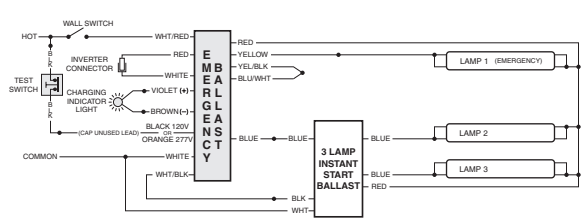
FIG C THREE (3) LAMP INSTANT START BALLAST
