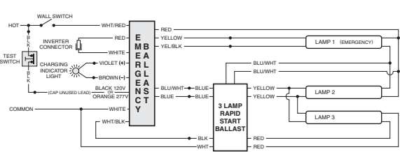
FIG D THREE (3) LAMP RAPID START BALLAST
