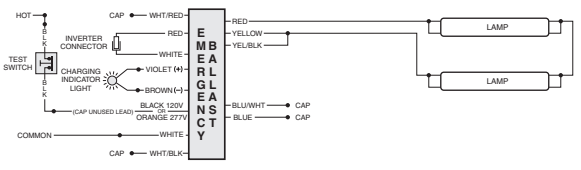
FIG M TWO (2) 17-40 W LAMPS WITHOUT AC BALLAST
