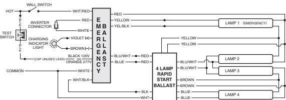
FIG F FOUR (4) LAMP RAPID START BALLAST
