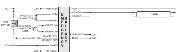
FIG L ONE (1) 17-215 W LAMP WITHOUT AC BALLAST
