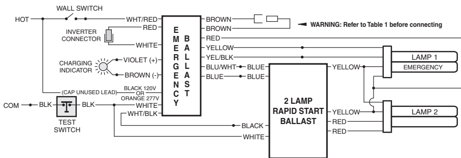
FIG H. TWO (2) 4-PIN COMPACT LAMP RAPID START BALLAST
