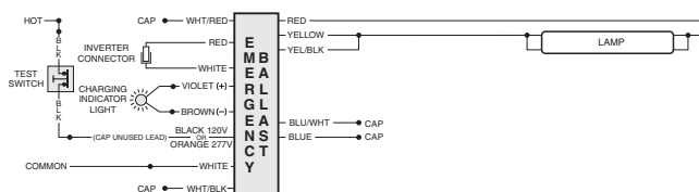
FIG 109 ONE (1) 17-40 W LAMP WITHOUT AC BALLAST
